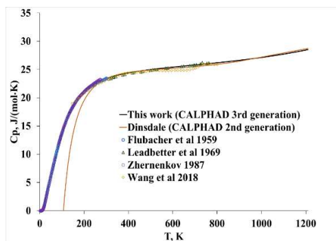
Experimental data and calculation results of heat capacity of pure crystalline germanium in the temperature range 0- T_{\text{fus}}
